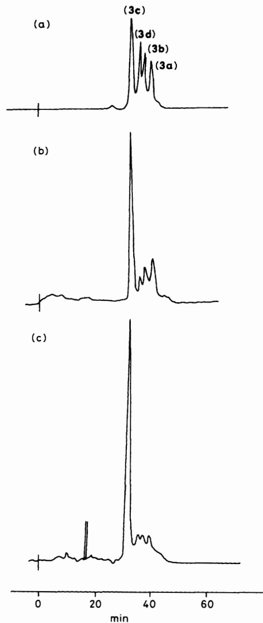
Figure 1. H.p.l.c. comparisons of (a) the four synthetic desethylaetioporphyryns (3a–d) with the corresponding petroporphyrin fractions from (b) Gilsonite and (c) Serpiano shale. (Conditions: 2 \times 10 \mu Perkin–Elmer ODS–HC–Sil–XI reversed phase silica columns, each 25 \text{ cm} \times 3 \text{ mm} i.d.; mobile phase, acetonitrile with flow rate 0.3 \text{ ml/min} and detector set at 400 \text{ nm} .)
